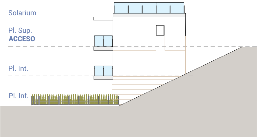
Alzado norte North elevation
